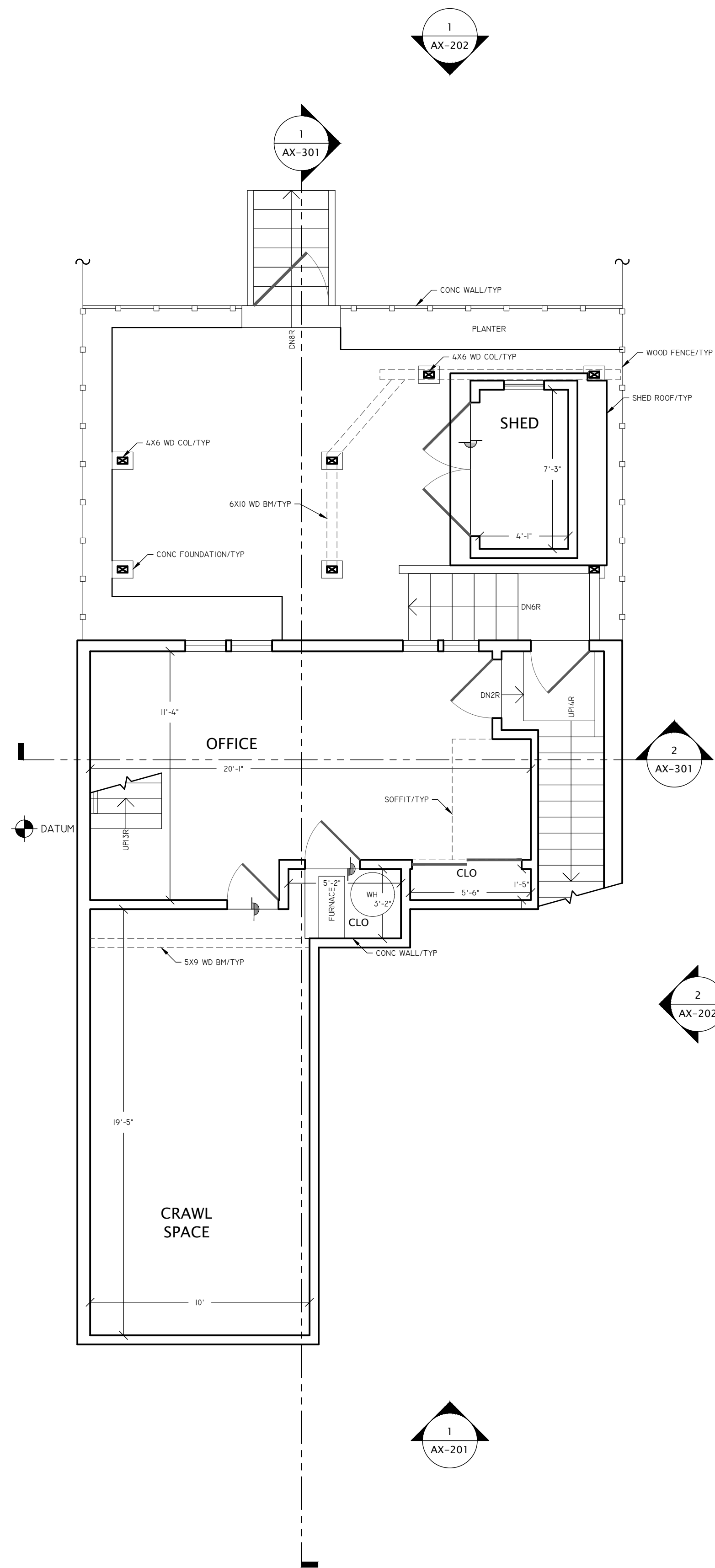
1 EXISTING LOWER LEVEL FLOOR PLAN 566 SQFT CROSS MEASURED AREA 357 SQFT MEASURED EXTERIOR SURFACES
