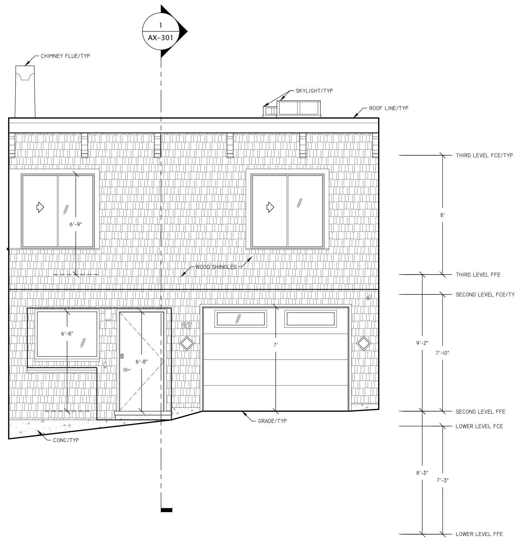
1 EXISTING NORTH ELEVATION
