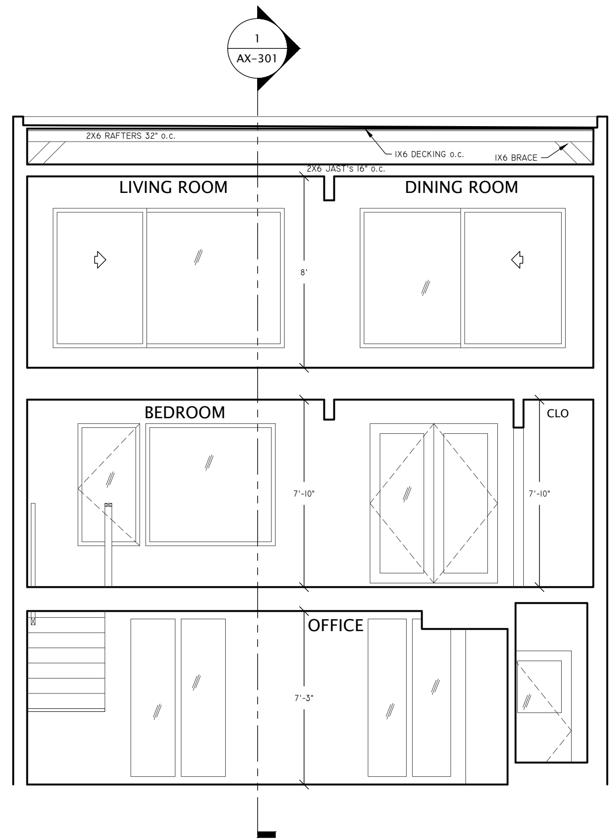
2 EXISTING CROSS SECTION
