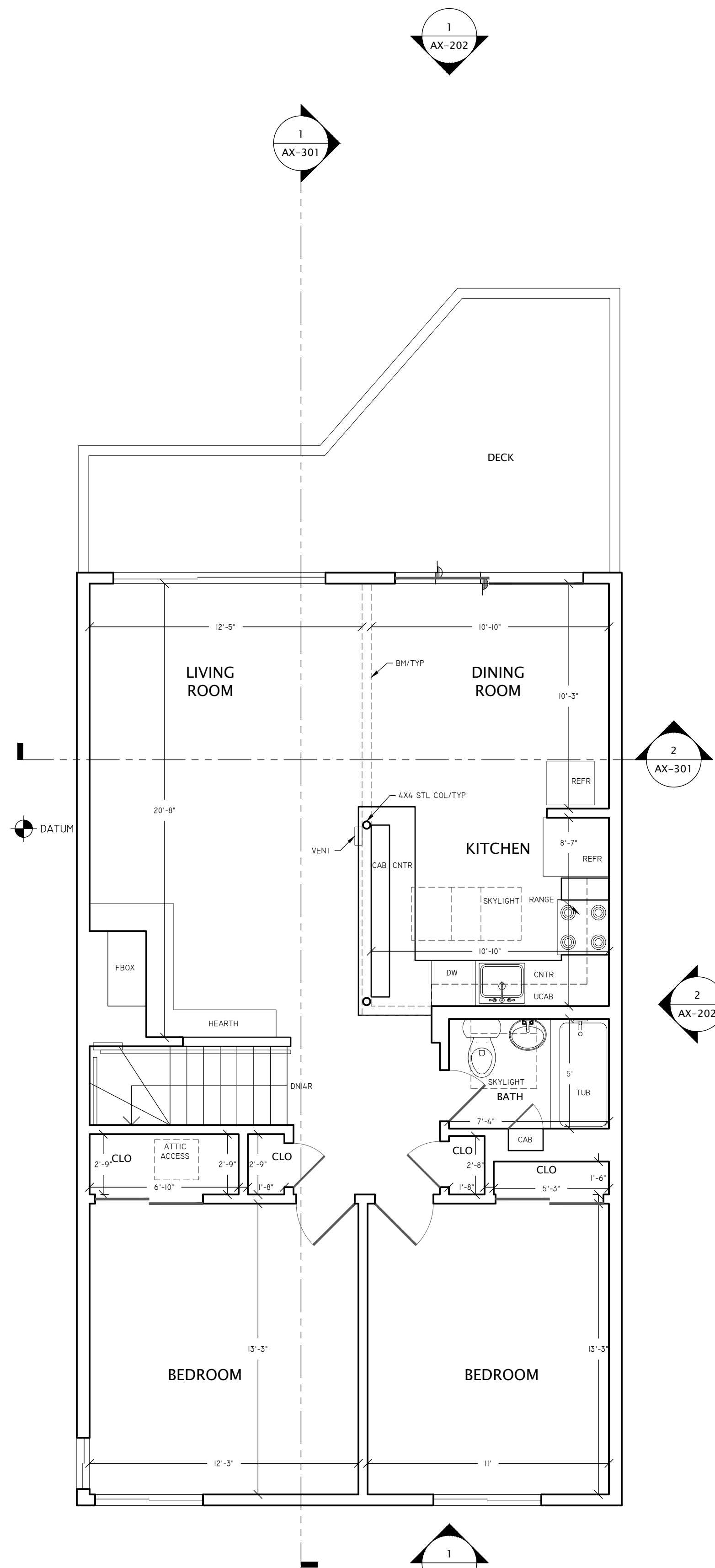
3 EXISTING SECOND LEVEL FLOOR PLAN 1,055 SQFT CROSS MEASURED AREA 218 SQFT MEASURED EXTERIOR SURFACES
