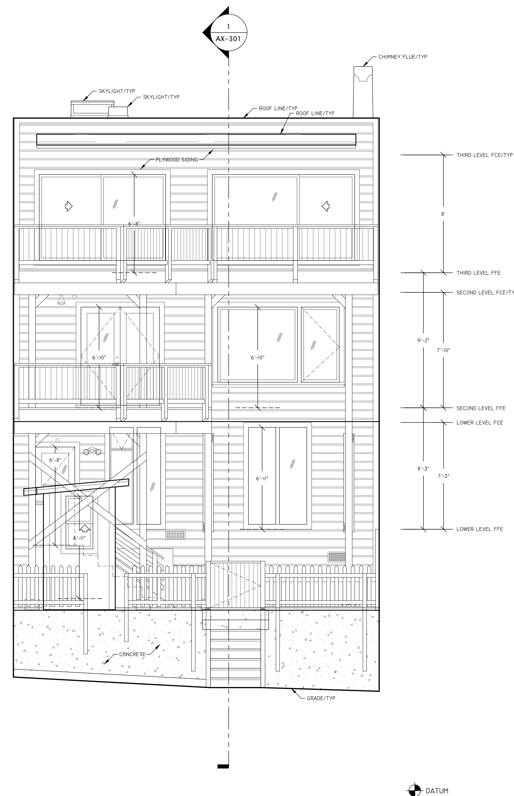
① EXISTING SOUTH ELEVATION
