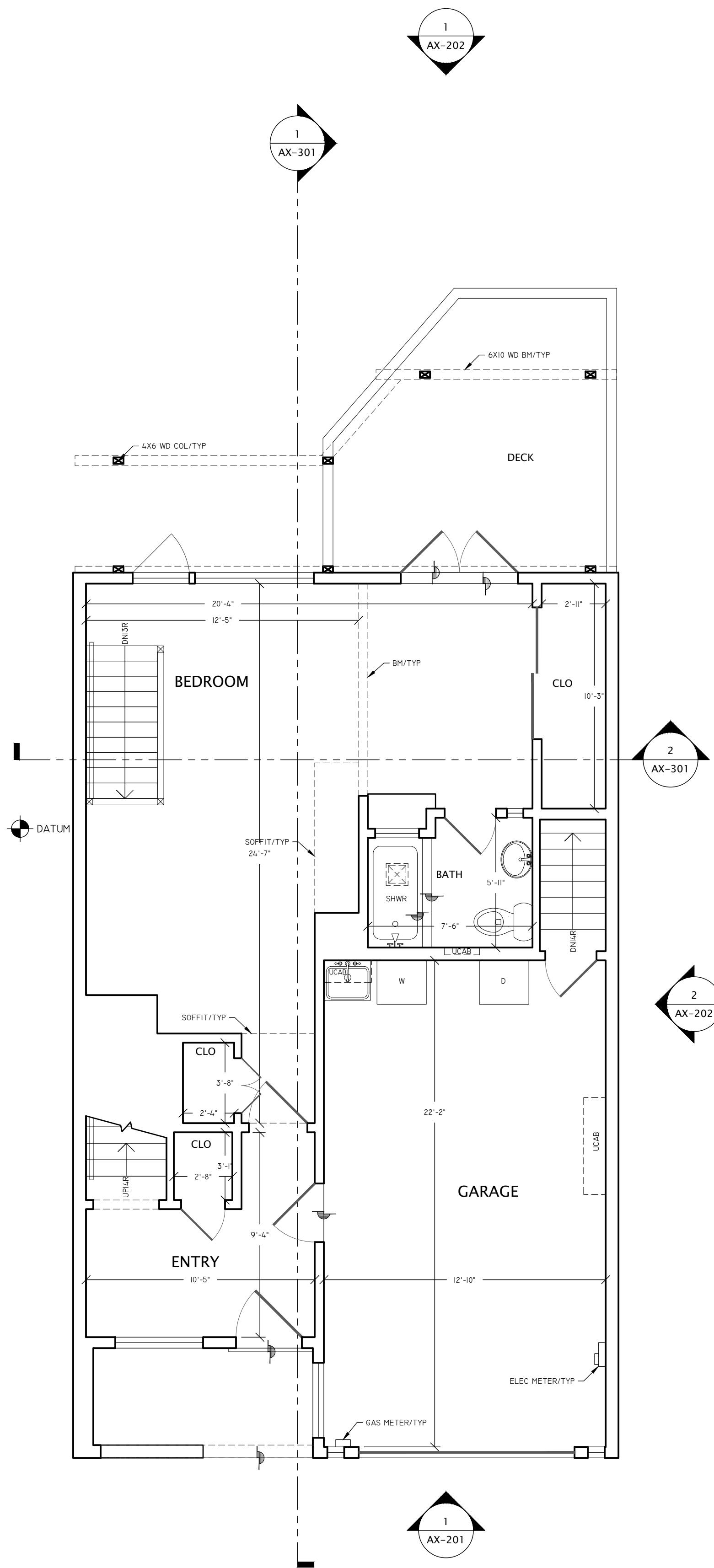
2 EXISTING ENTRY LEVEL FLOOR PLAN 955 SQFT CROSS MEASURED AREA 200 SQFT MEASURED EXTERIOR SURFACES
